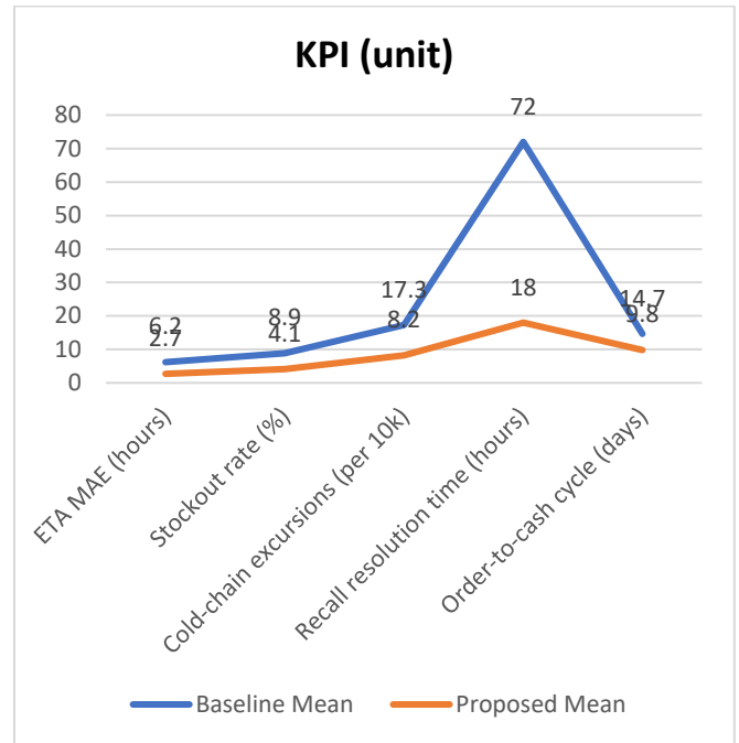
Figure-3. KPI Comparison: Baseline vs. Blockchain+AI Scenario
